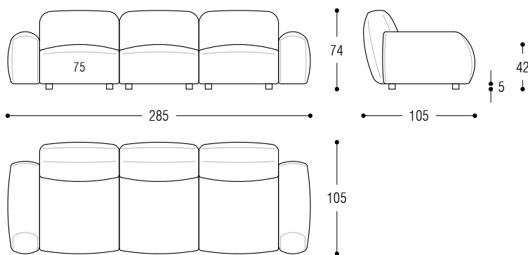
Element cm 105 left + central element cm 75 + element 105 right
