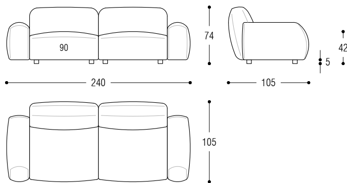
Element cm 120 left + element cm 120 right
