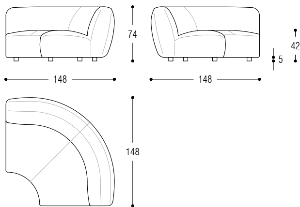
Corner element cm 148x148
